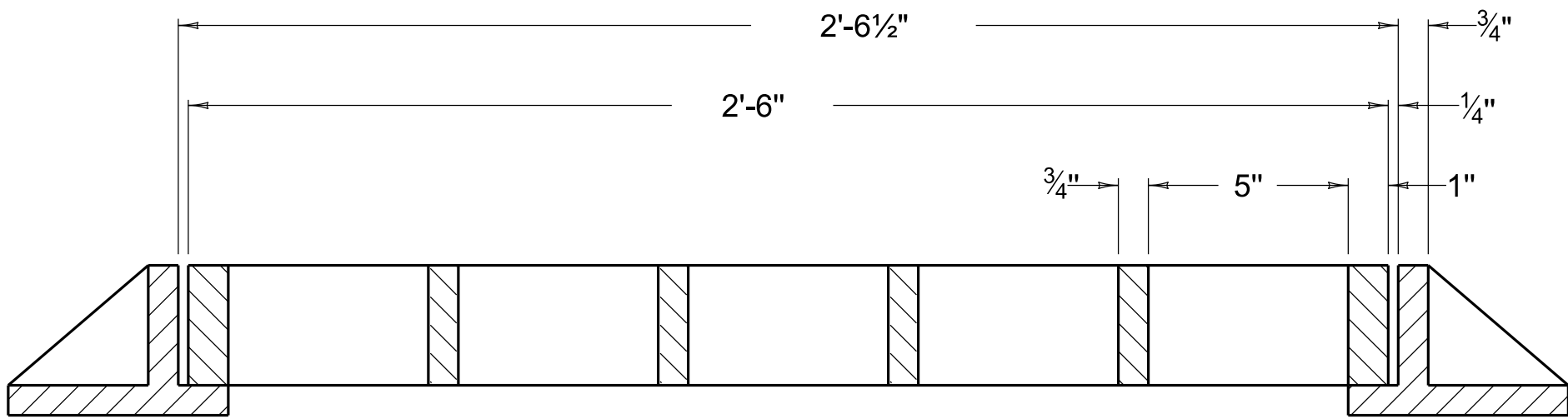
SECTION B-B
